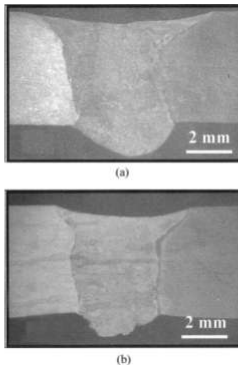
Figure 4. —Weld bead geometry for validating: (a) apply Taguchi method, DWR = 0.785; (b) apply proposed approach, DWR = 0.915.
